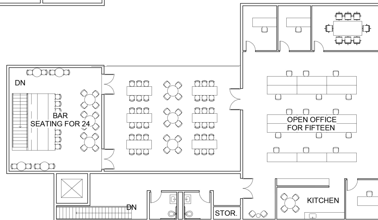
1 Level 2 1/16" = 1'-0"
