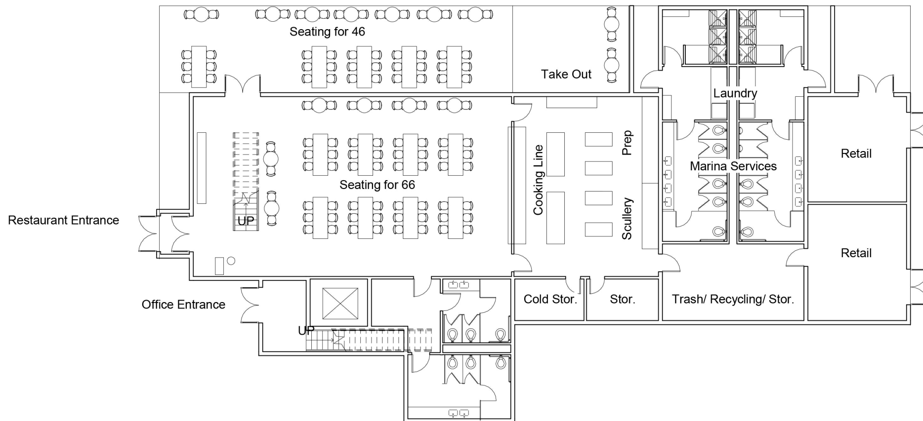
1 Level 1 1/16" = 1'-0"
